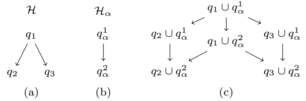
Fig. 1: Rewriting graphs of Example 4.
